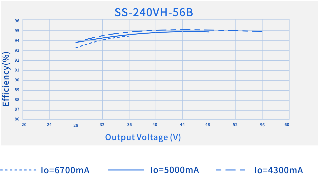
Efficiency Vs. O/P Voltage (Vin=277Vac)
